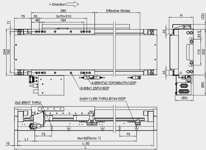
Dimensions and weight of the linear motor stages LMX1L-S37-1-xxxx-G2A0 and LMX1L-S37L-1-xxxx-G2A0 with cover
