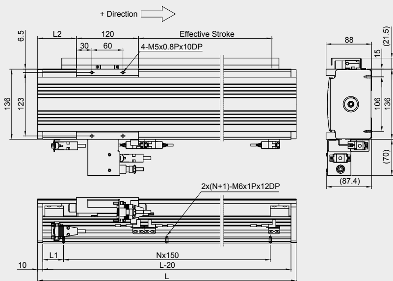
Dimensions and weight of the linear motor stage LMX1E-TB2-1-xxxx-G2A0
