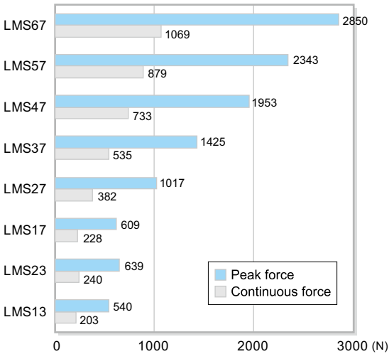
Force Chart for Linear Motors, LMS Series
