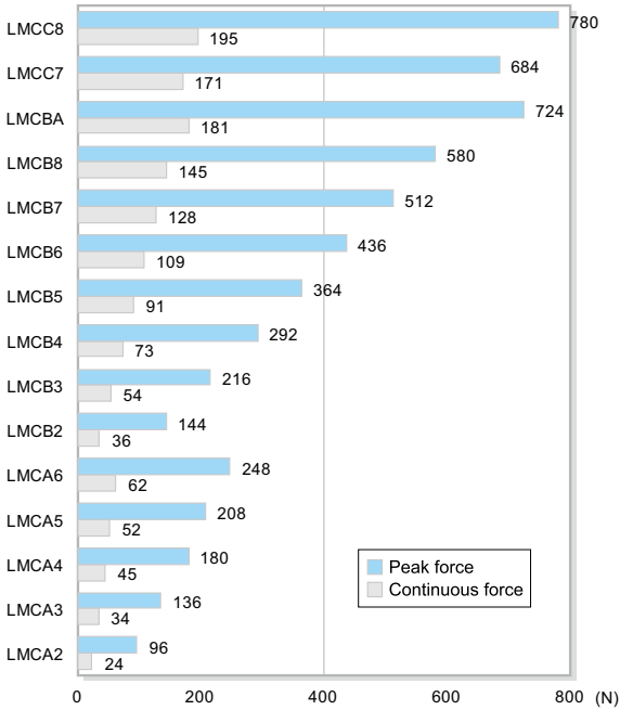
Force Chart for Linear Motors, LMCA,LMCB,LMCC Series
