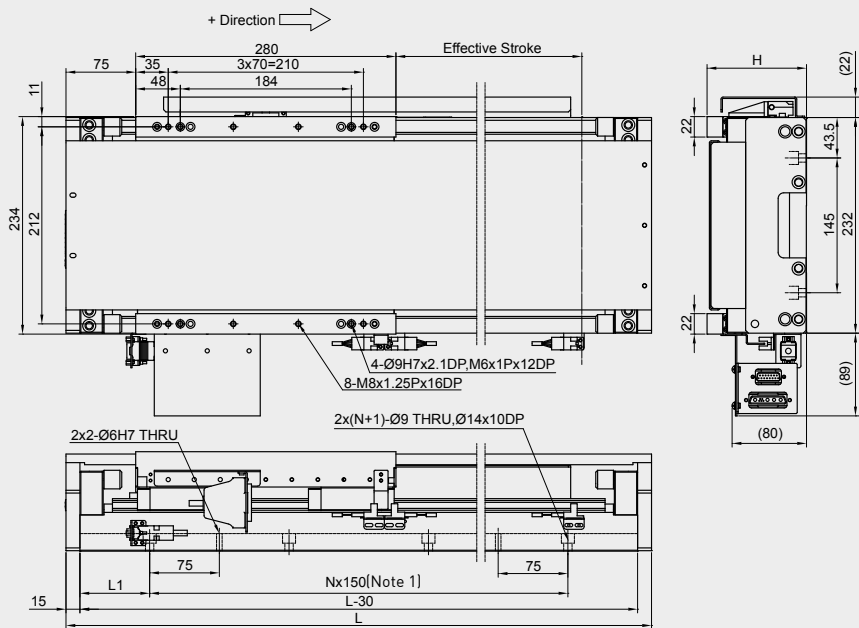
Dimensions and weight of the linear motor stages LMX1L-S47-1-xxxx-G2A0 and LMX1L-S47L-1-xxxx-G2A0 with cover
