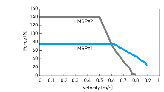
LMSP series F-V Curve
