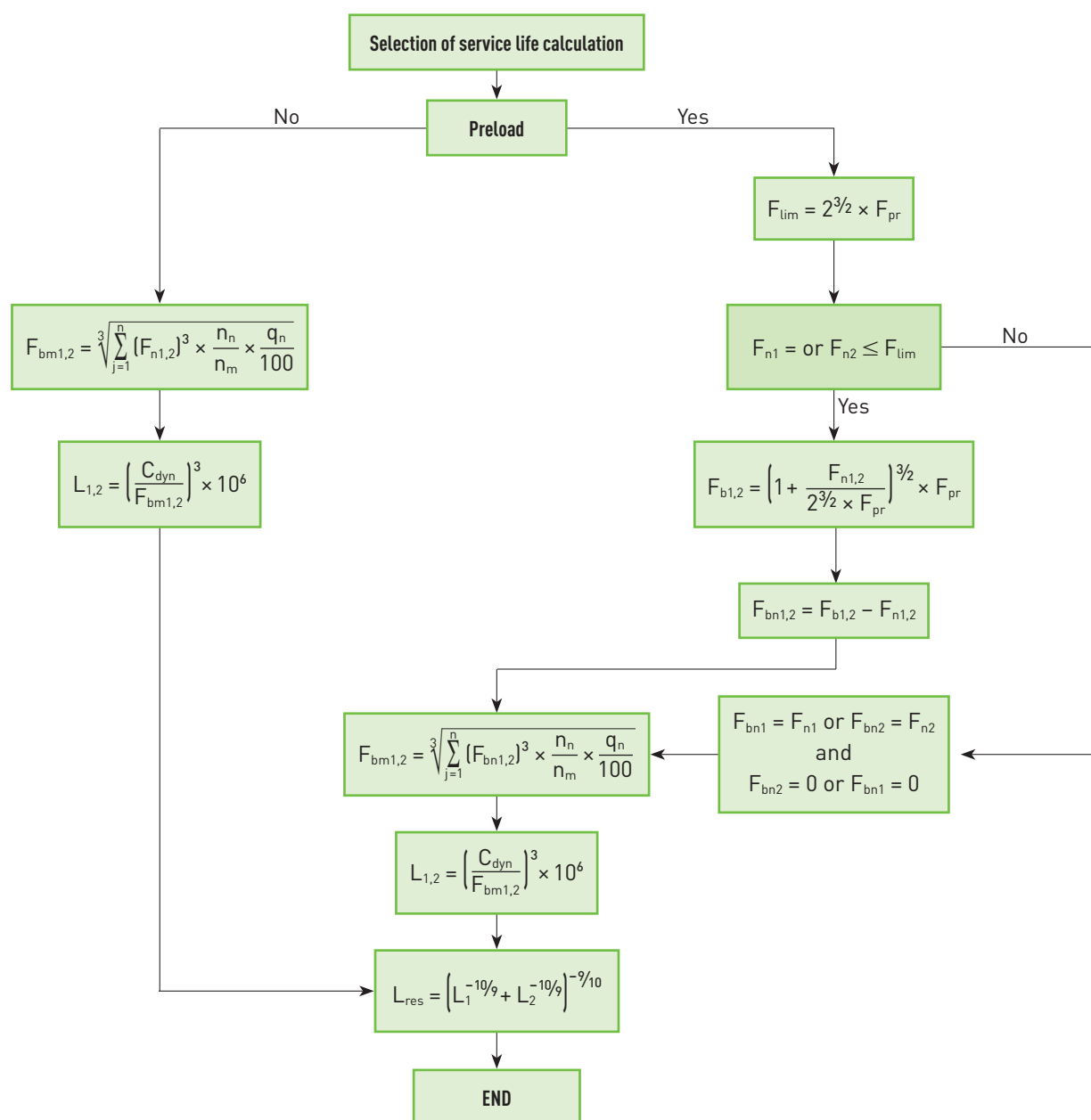
Flow chart for calculating service life
