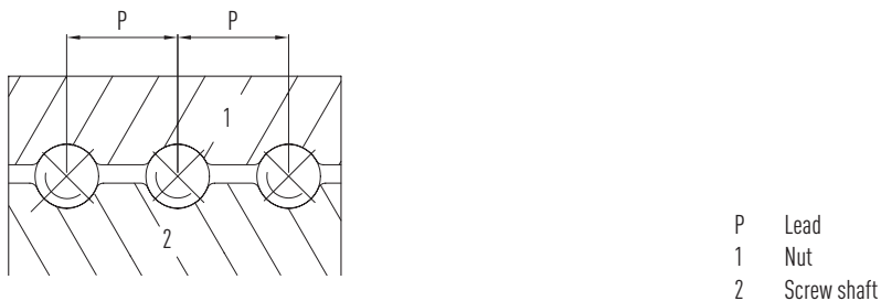
Fig. 3.16 Preload from ball size
